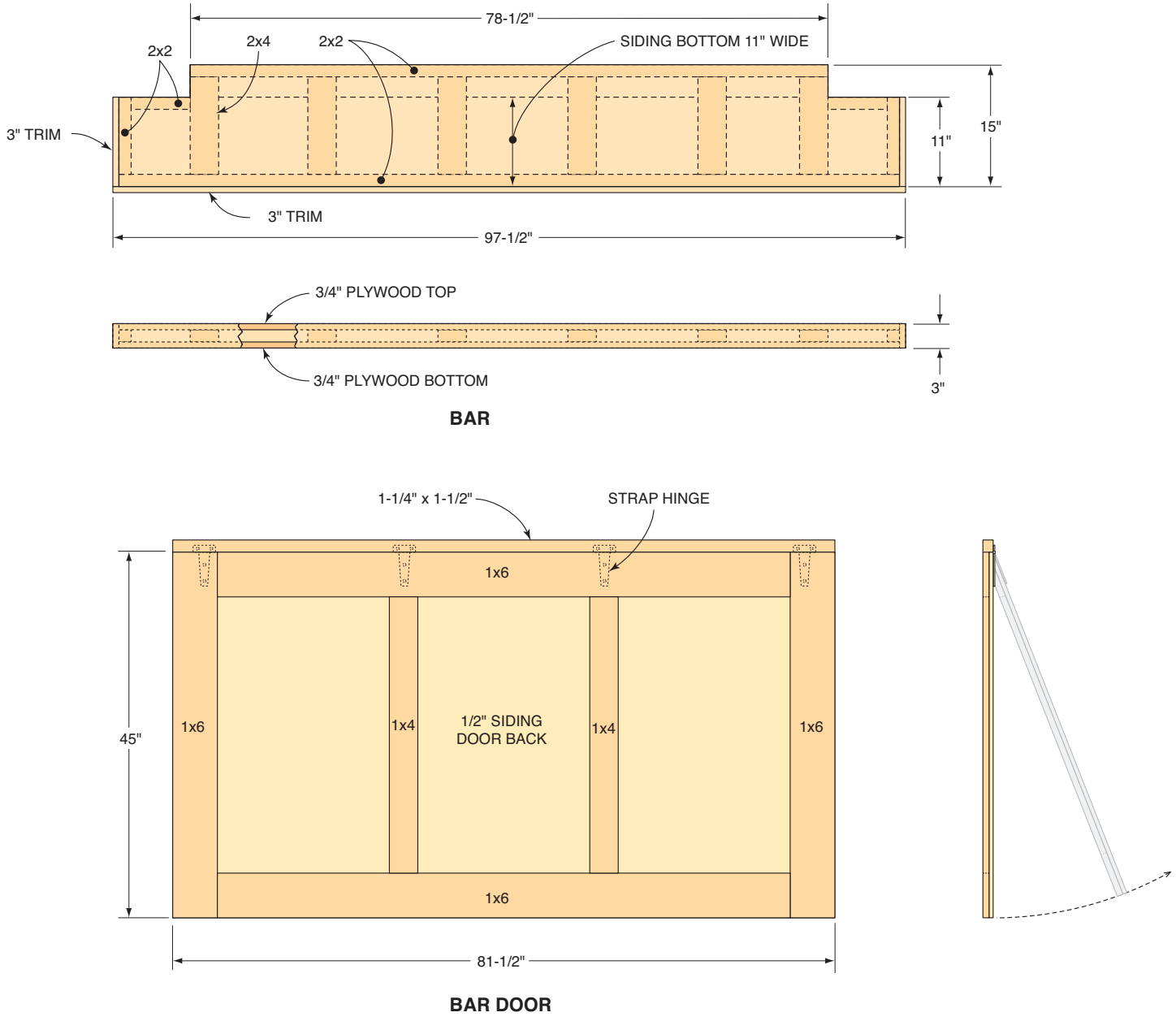
Figure P Bar and Bar Door Construction
