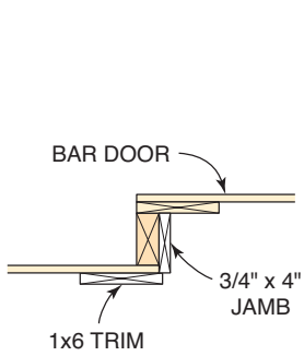
SECTION A-A (SEE FIGURE S)
