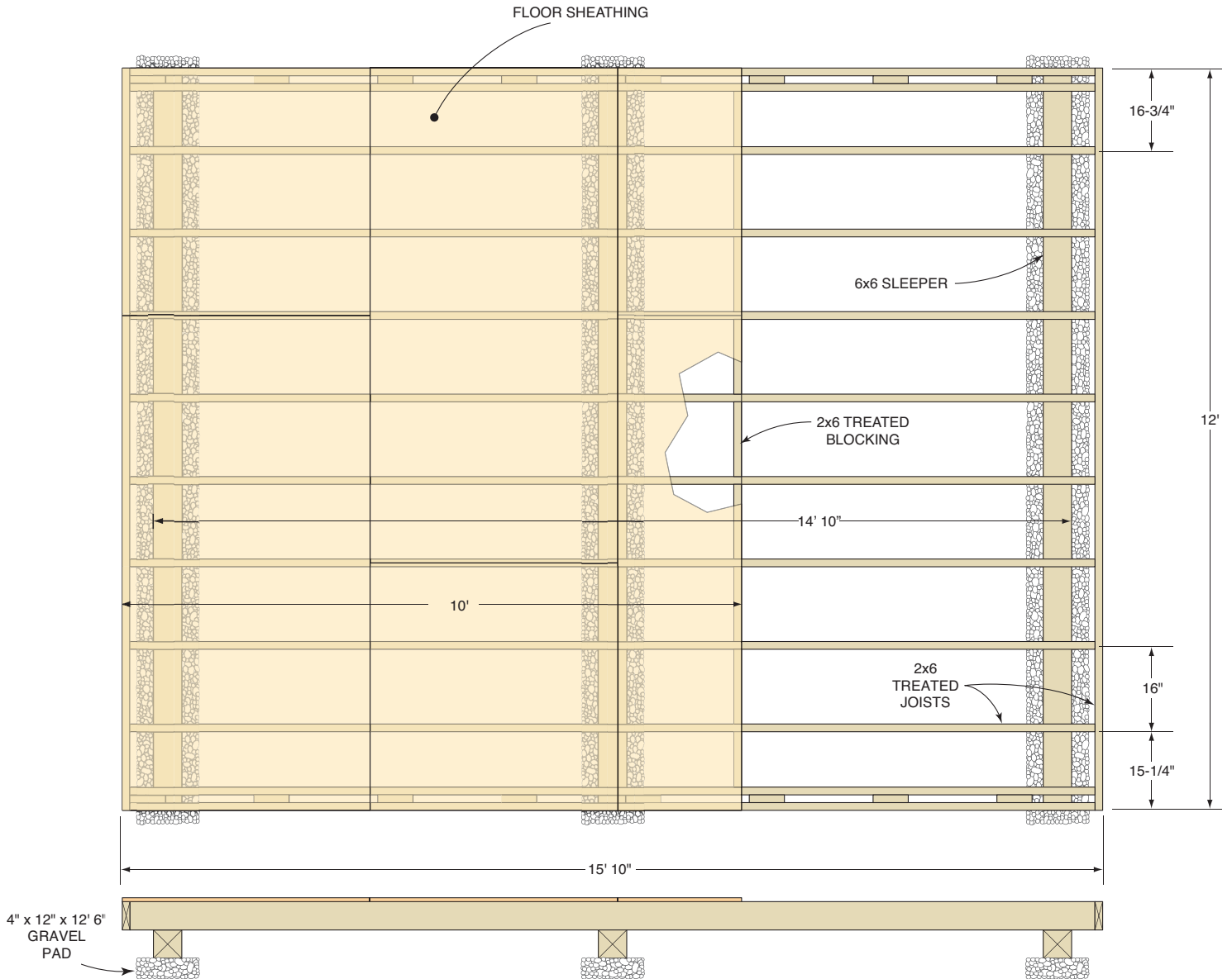
Figure B Floor Framing and Flooring
