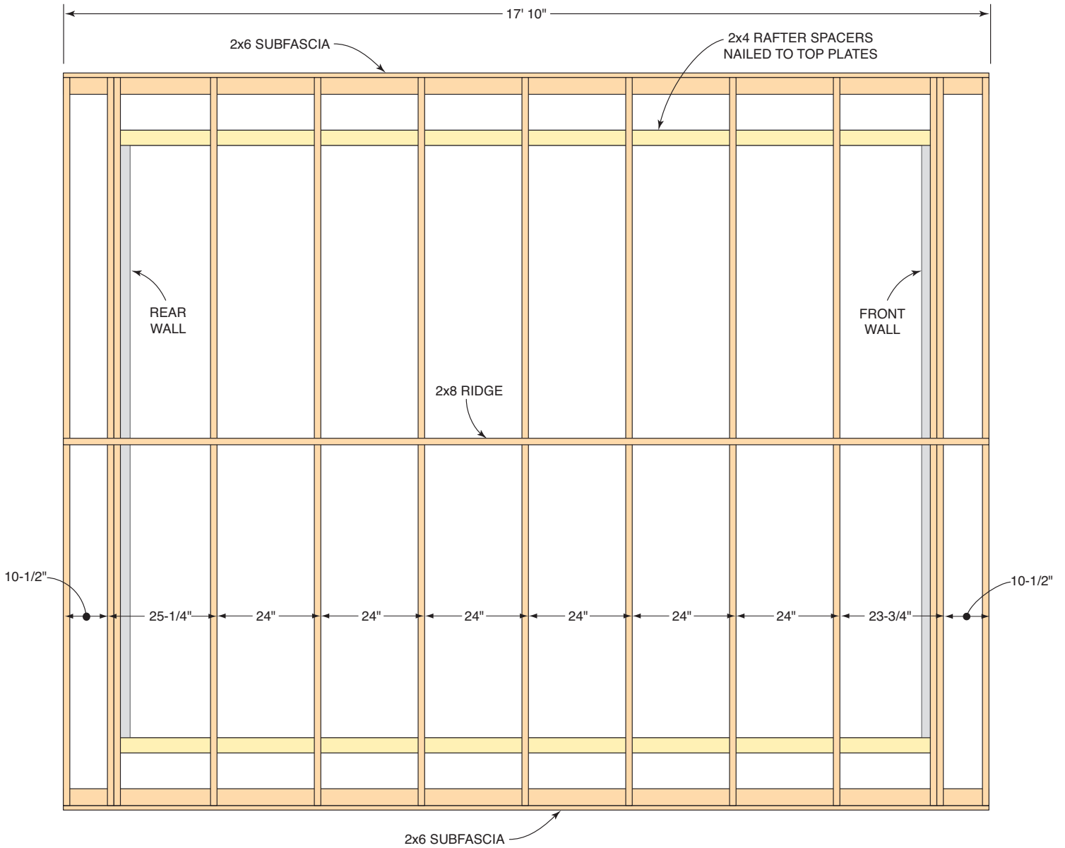
Figure K Rafters Spacing Plan View
