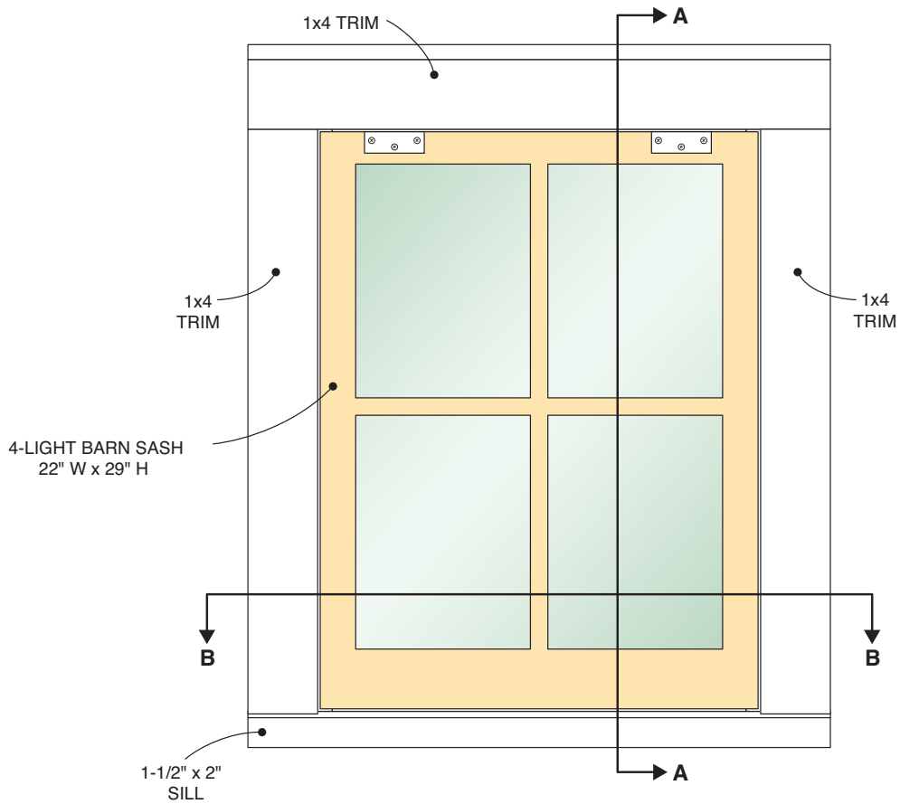
Figure Q Front Window Details
