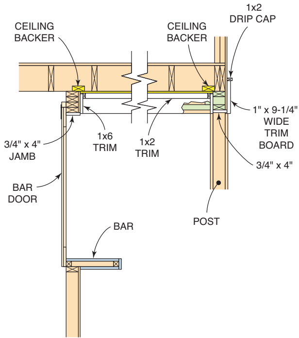
SECTION B-B (SEE FIGURE S)
