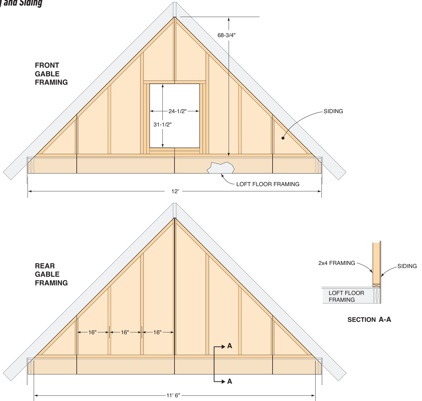
Figure L Front and Rear Gables Framing and Siding
