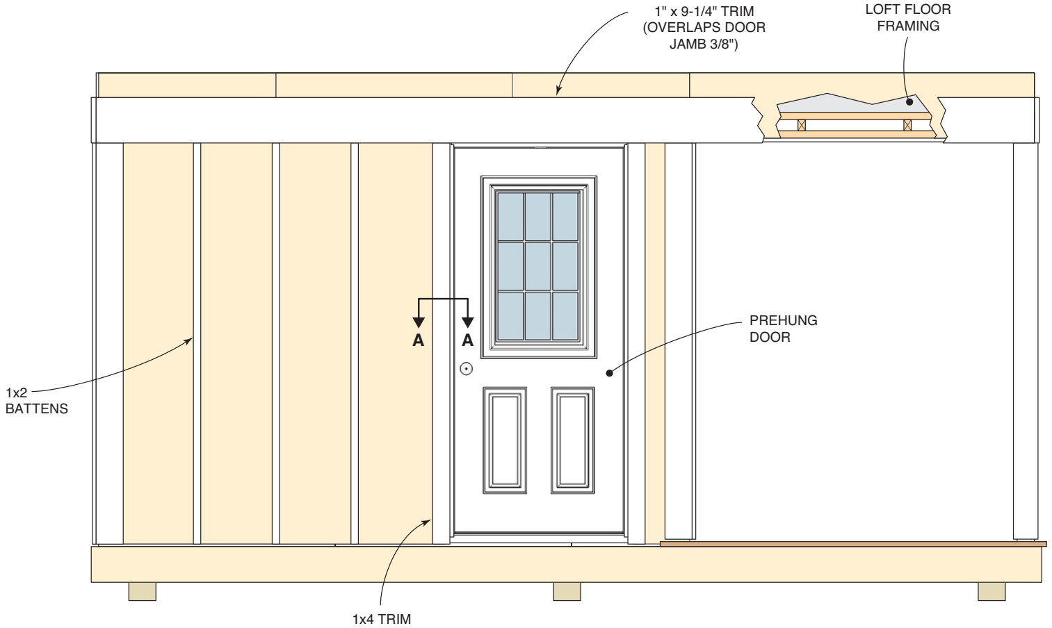
Figure V Left Side Wall
