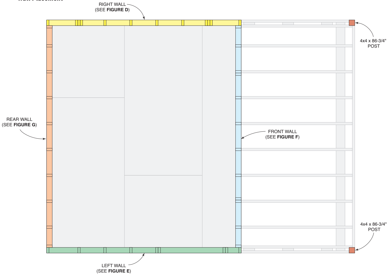
Figure C Wall Placement
