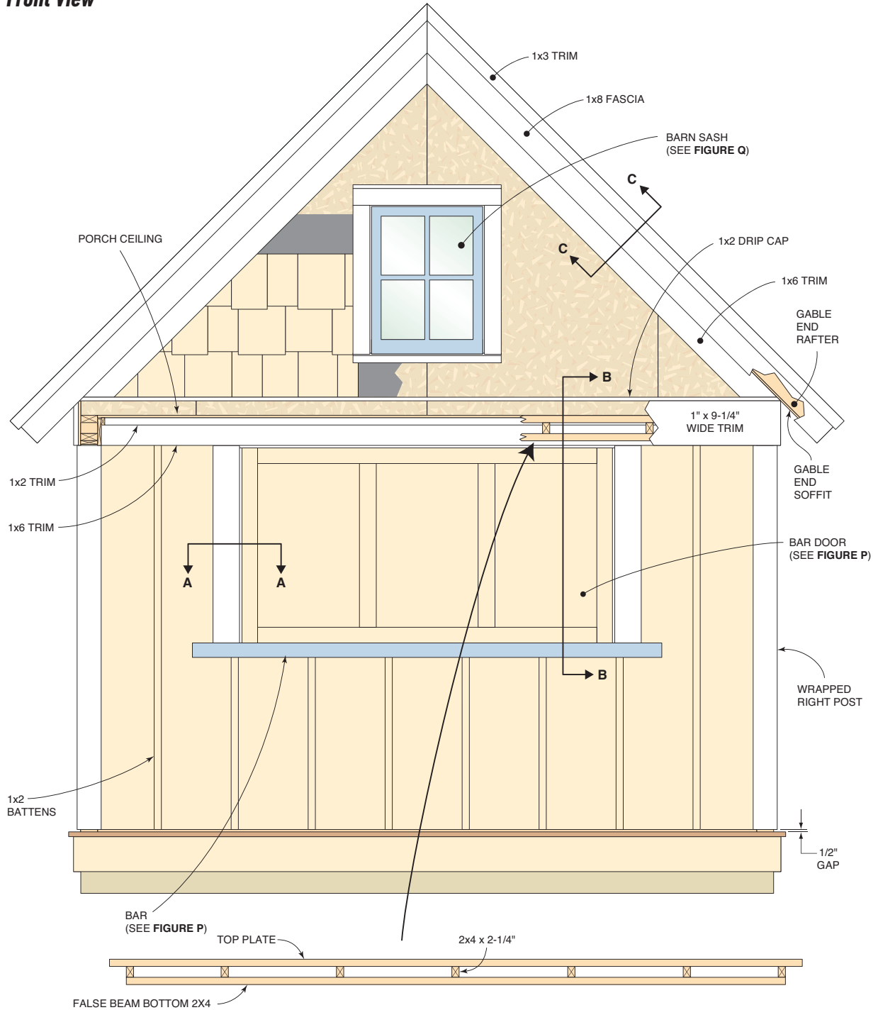
Figure S Front View
