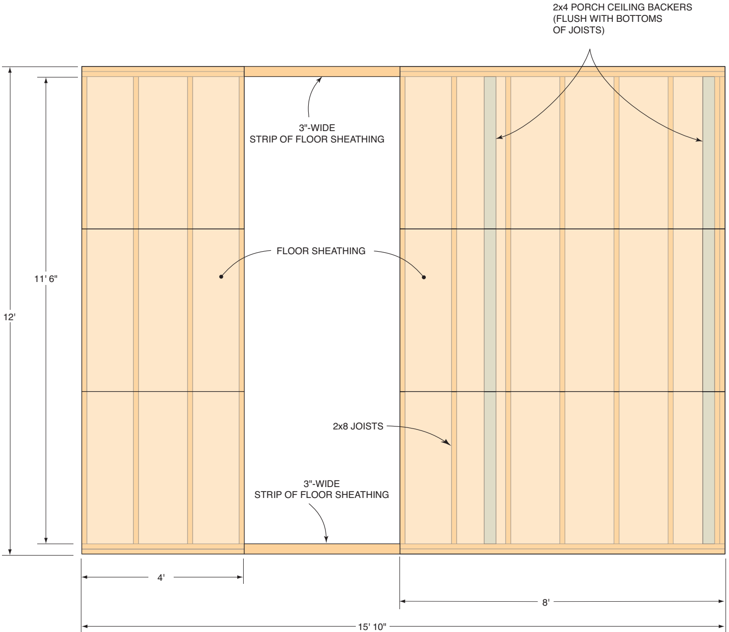
Figure H Attic Joists Framing and Flooring
