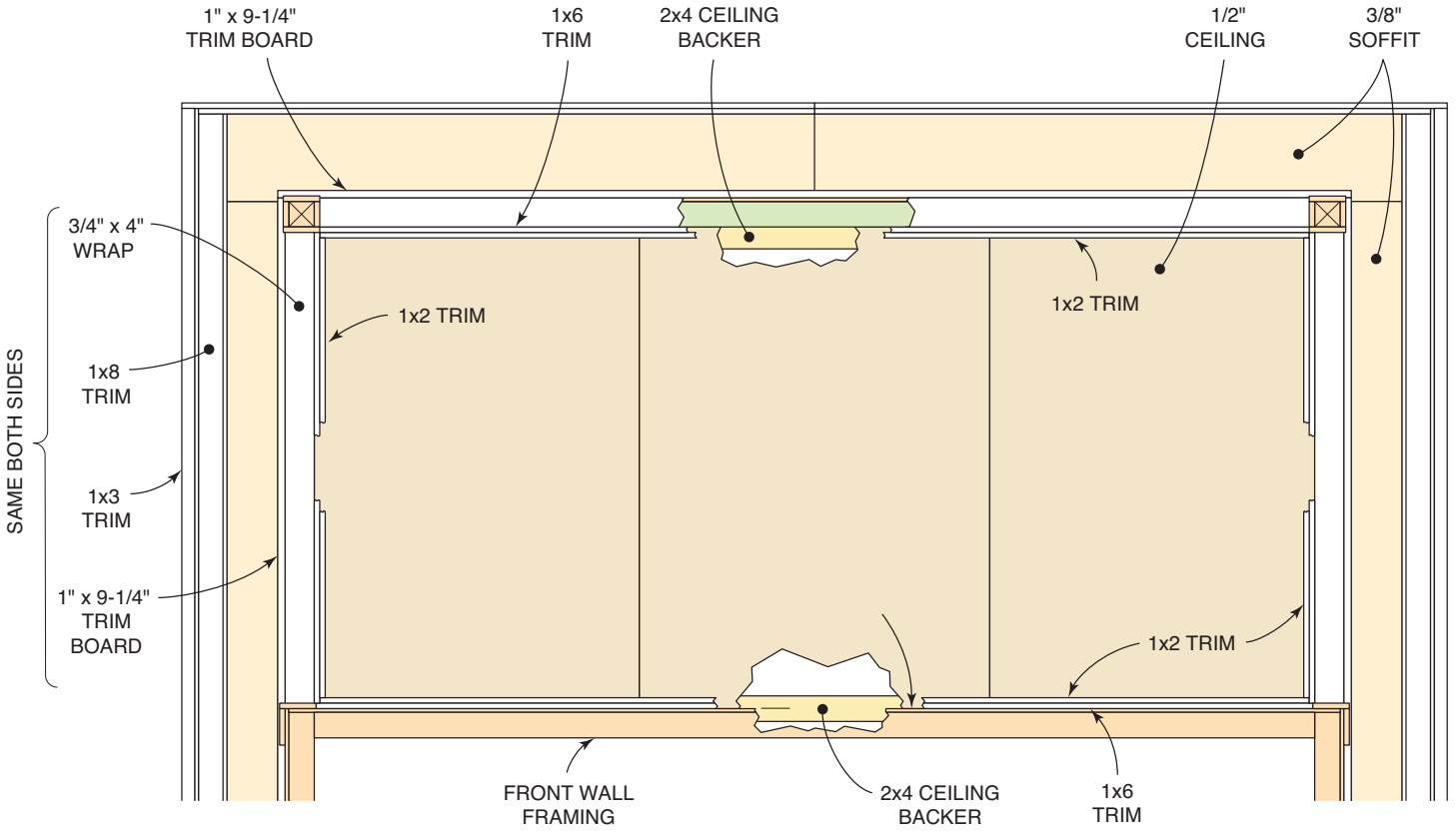
VIEW LOOKING UP
