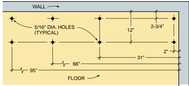
Fig. C Hole location for pins (top view)
